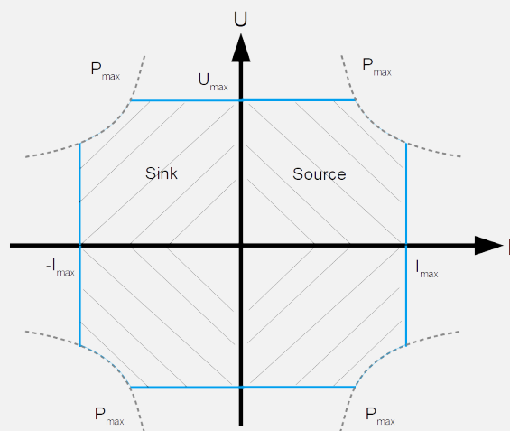
Figure 2. Maximum power within a voltage range of 0 V – U_{max} (4-QS system).
